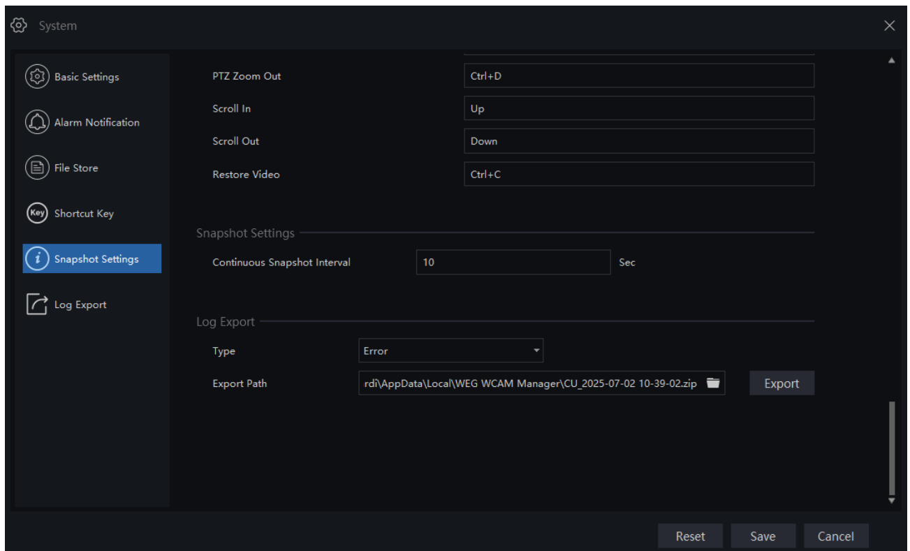
Figure 4-5: Capture and Log Export Configuration
